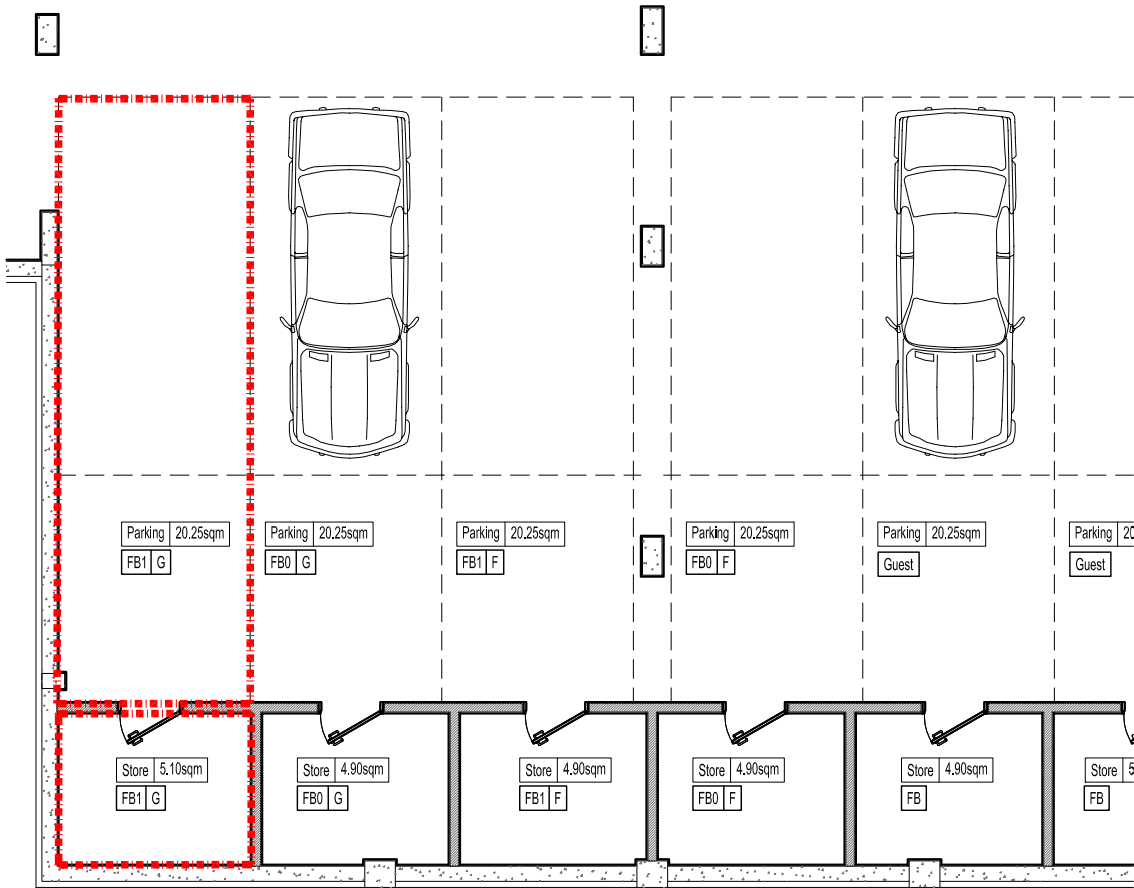
Parking level 1/100 scale
